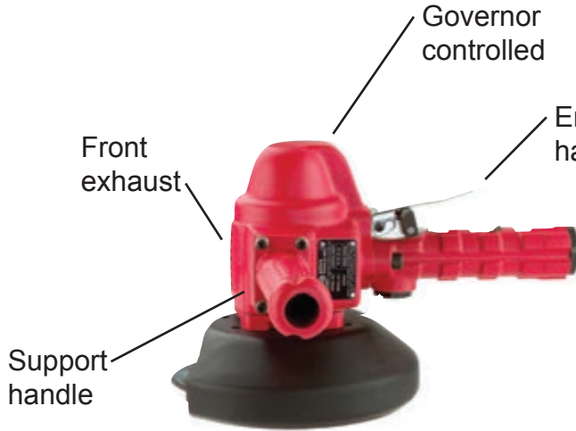
VG20AL-60D7 Type 27 Wheel Grinder
