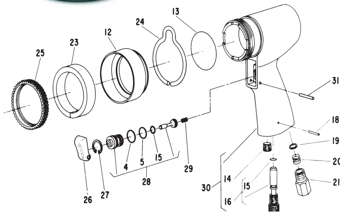
NON-REVERSING HANDLE ASSEMBLY (SERIAL NO'S. STARTING WITH "B" & "D")
