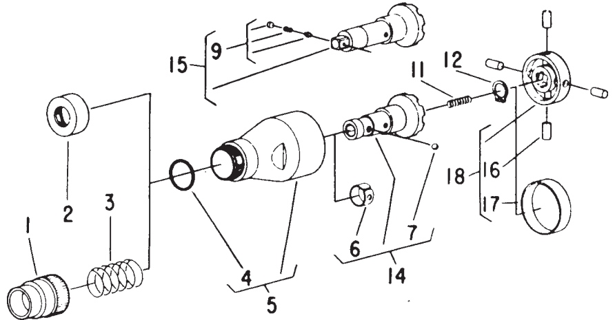
POSITIVE CLUTCH
