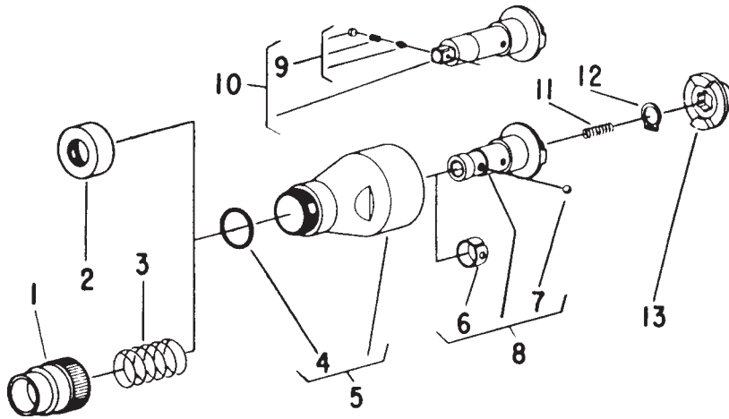
DIRECT CLUTCH
